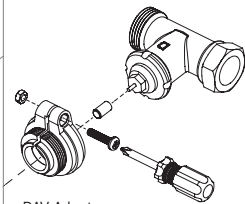
RAV Adapter
